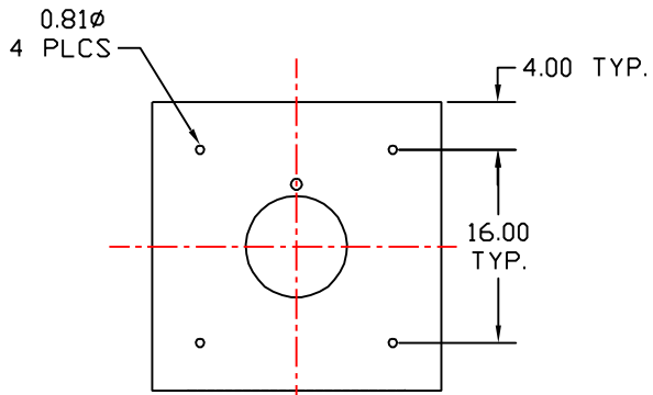
LIFT MOUNT PLATE DETAIL
